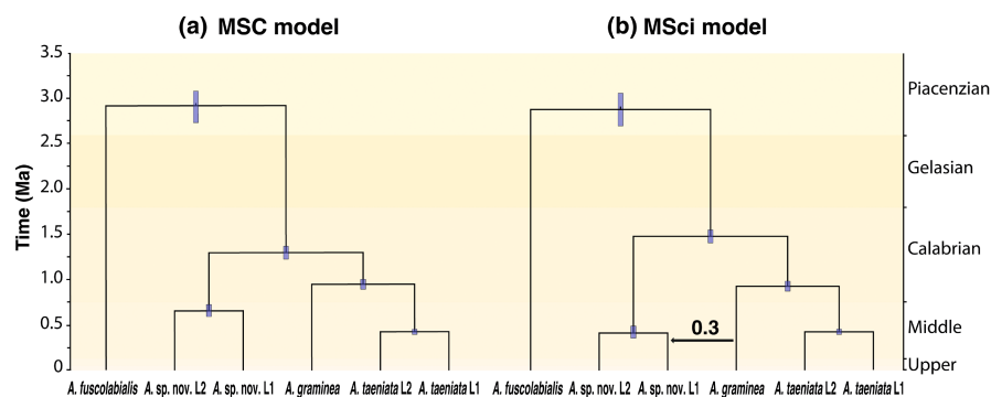
FIGURE 3 Time-calibrated species trees of Abronia taeniata – graminea complex from central Mexico estimated using BPP under (a) the multispecies coalescent (MSC) model and (b) the multispecies coalescent model with introgression (MSCi). Bars on nodes indicate 95% highest posterior densities (HPD) for divergence time estimates. Geologic ages within the Pliocene (Piacenzian) and Quaternary (Gelasian, Calabrian, Middle and Upper) periods are indicated in the right y-axis.
