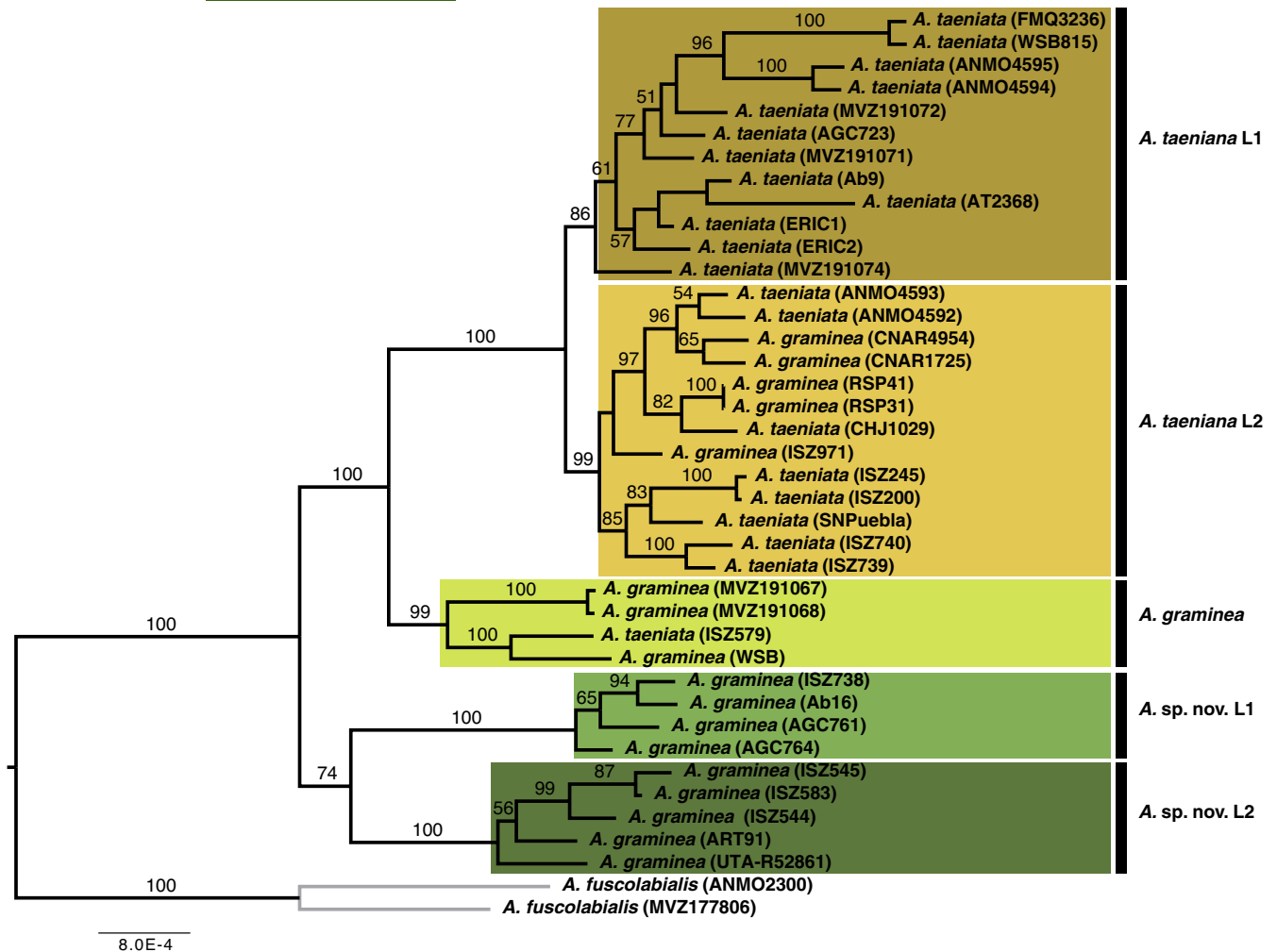
FIGURE 2 Maximum likelihood consensus tree based on RAXML analyses of arboreal alligator lizards of the Abronia taeniata – graminea species complex from central Mexico. Analyses are based on the F96m80 matrix, that is, minimum number of samples with data for a locus to be included in the alignment = 80%. Bootstrapping support values are indicated next to their respective branches. Individual codes as described in Table S1.
