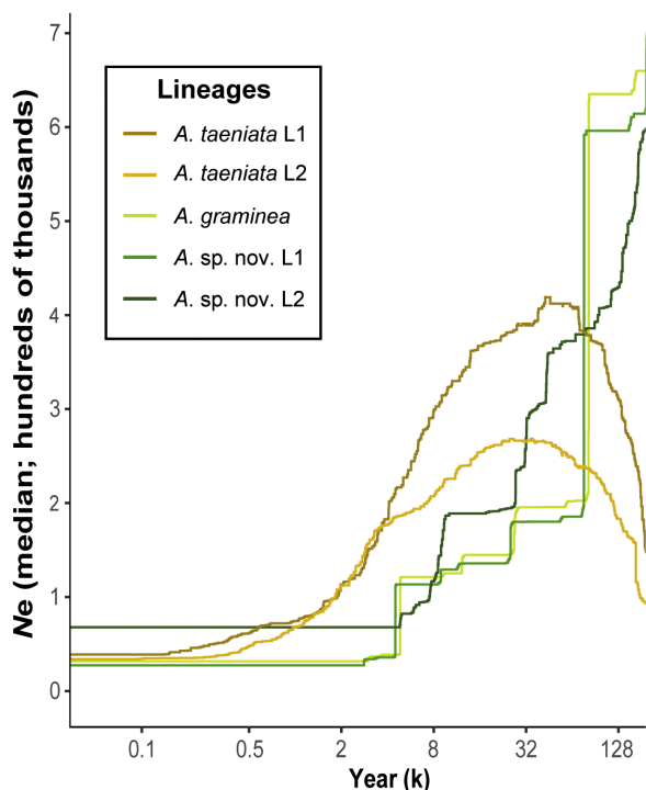
FIGURE 4 Demographic history of each lineage of Abronia taeniata – graminea species complex from central Mexico estimated using STAIRWAY PLOT 2. Panels show median effective population sizes ( N_e ) over time (x-axis in a logarithmic scale).
