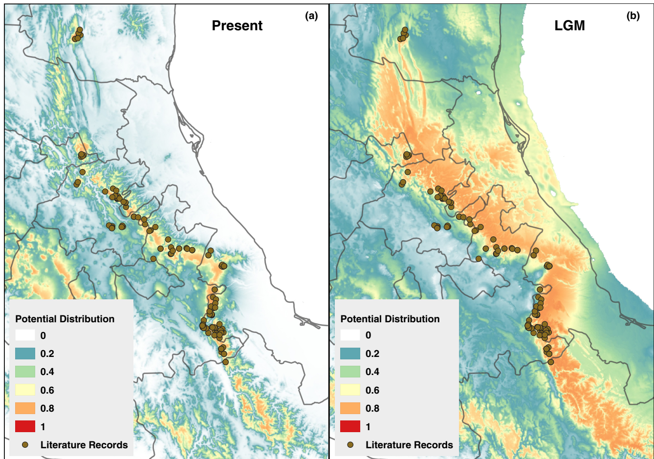
FIGURE 5 Present (a) and LGM (b) projections of the environmental niche model (ENM) in MAXENT for arboreal alligator lizards of the Abronia taeniata-graminea species complex from central Mexico. Dots represent all known localities of specimens deposited in herpetological collections. Maps in Plate Carrée projection. LGM, Last Glacial Maximum.
